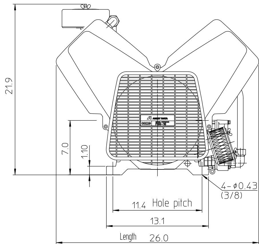
Back view
