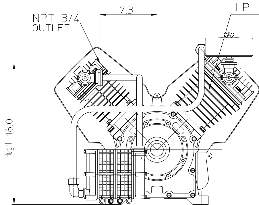
Back view
