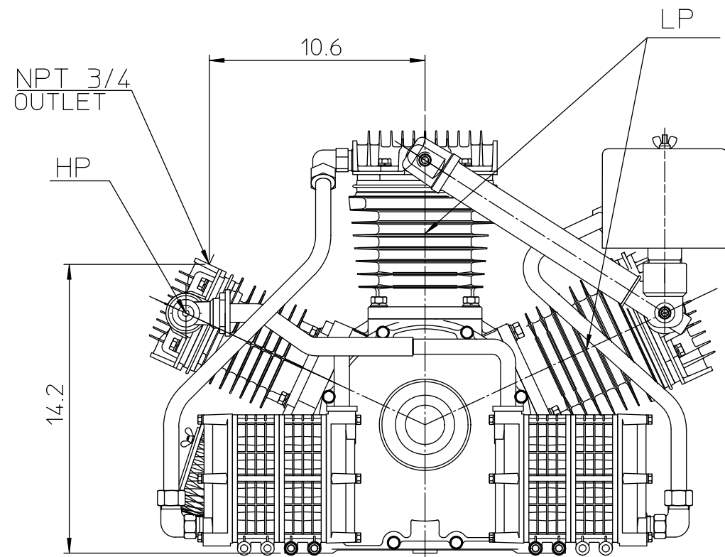
Back view
